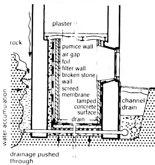
⑩ Damp-proofing from inside with partially inaccessible outer walls
